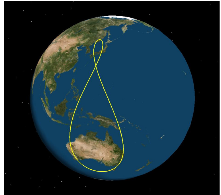
Asymmetry orbit in the shape of a 'figure 8' ©JAXA
